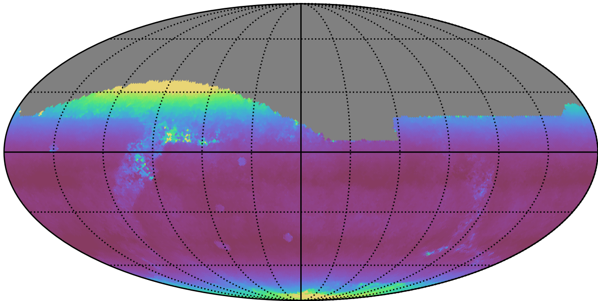
ddf_loaded_half_fl8_v3.4_10yrs All sky z band: Median airmass
