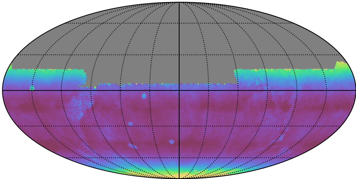
ddf_loaded_half_fl8_v3.4_10yrs All sky y band: Median airmass
