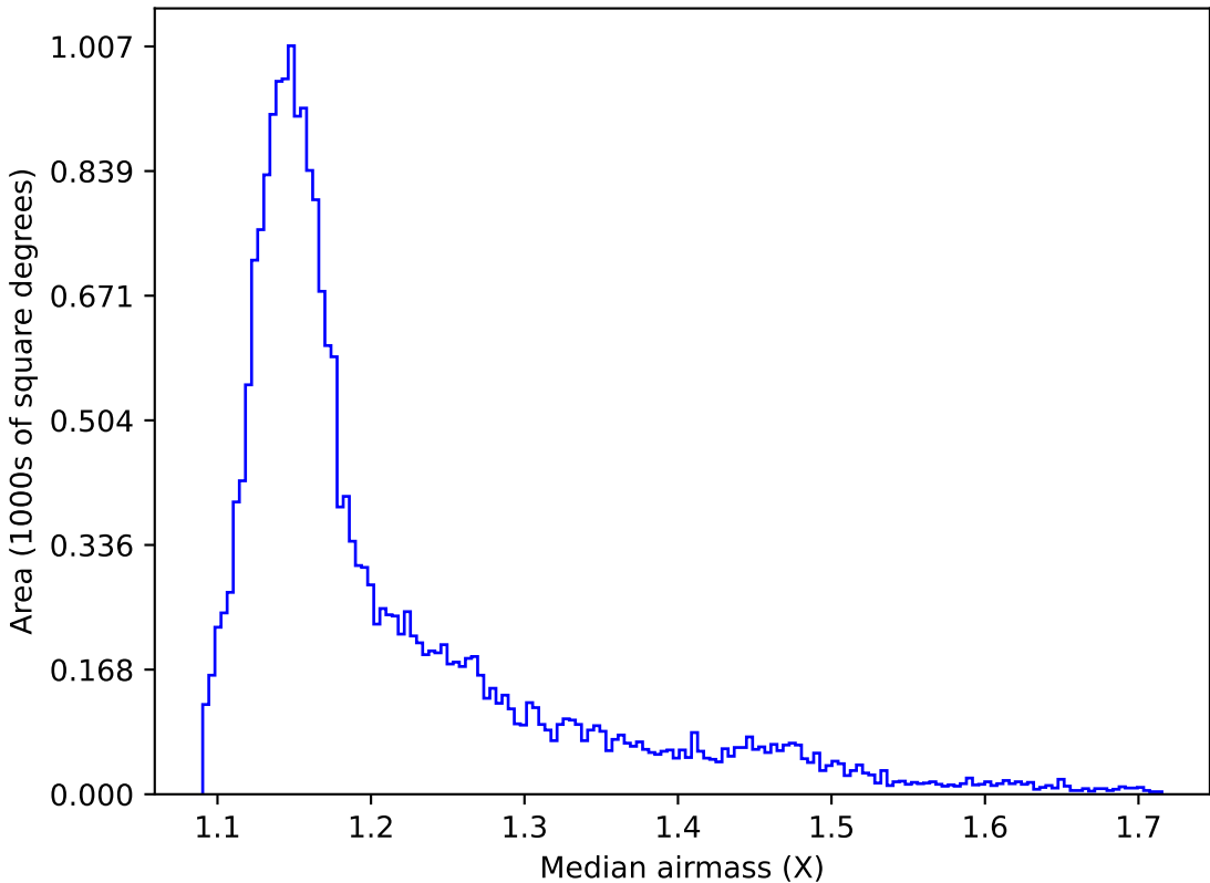
ddf_loaded_half_fl8_v3.4_10yrs All sky y band: Median airmass
