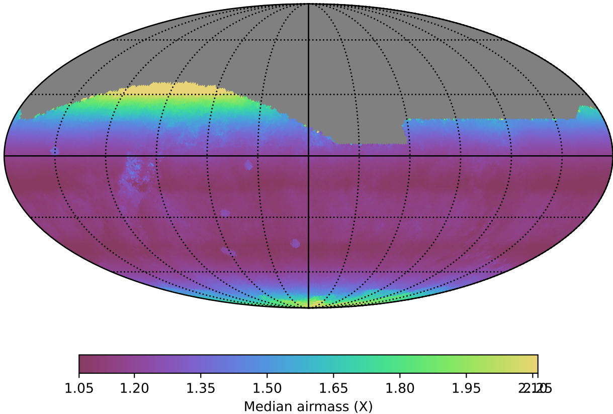
ddf_loaded_half_fl8_v3.4_10yrs All sky r band: Median airmass
