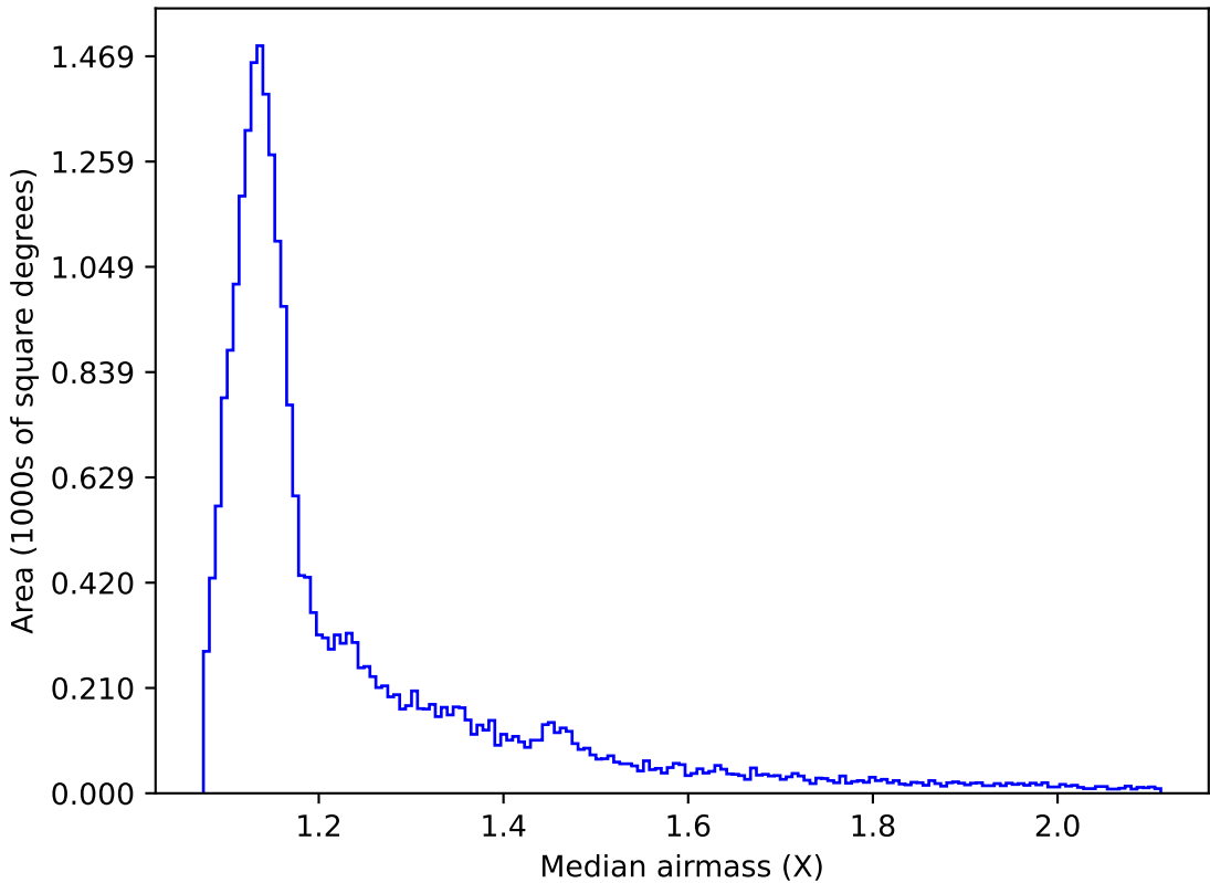
ddf_loaded_half_fl8_v3.4_10yrs All sky r band: Median airmass
