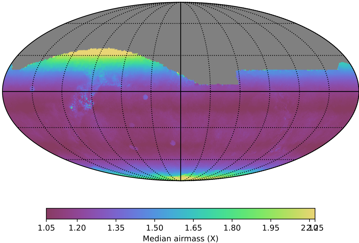
ddf_loaded_half_fl8_v3.4_10yrs All sky i band: Median airmass
