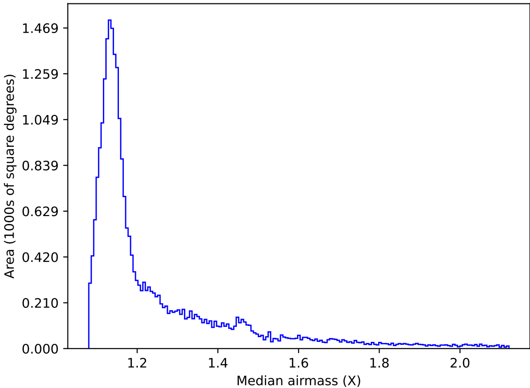
ddf_loaded_half_fl8_v3.4_10yrs All sky i band: Median airmass
