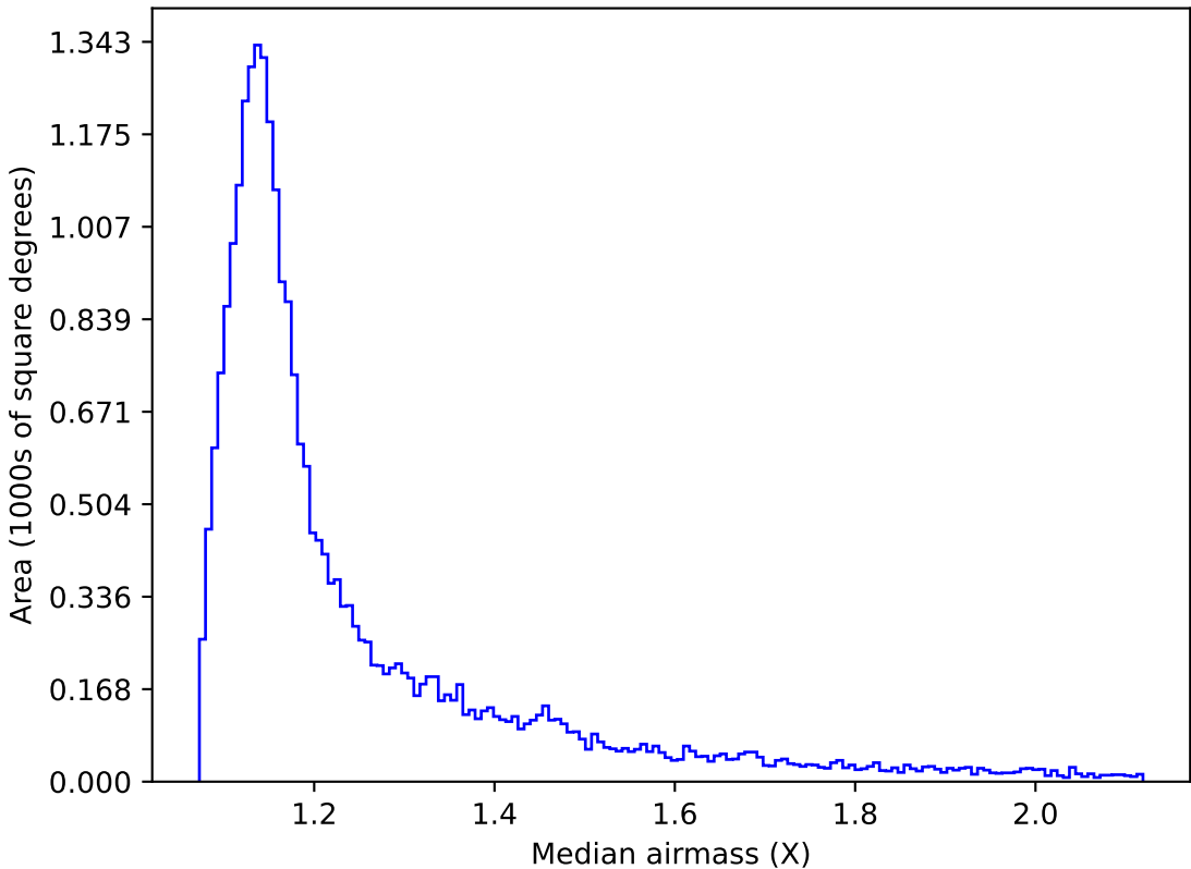
ddf_loaded_half_fl8_v3.4_10yrs All sky g band: Median airmass
