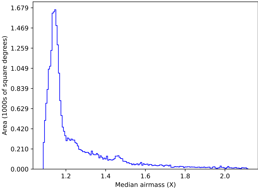
ddf_loaded_half_fl8_v3.4_10yrs All sky all bands: Median airmass
