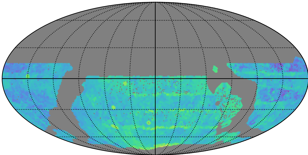
ddf_loaded_half_fl8_v3.4_10yrs WFD z band: Median Season Length
