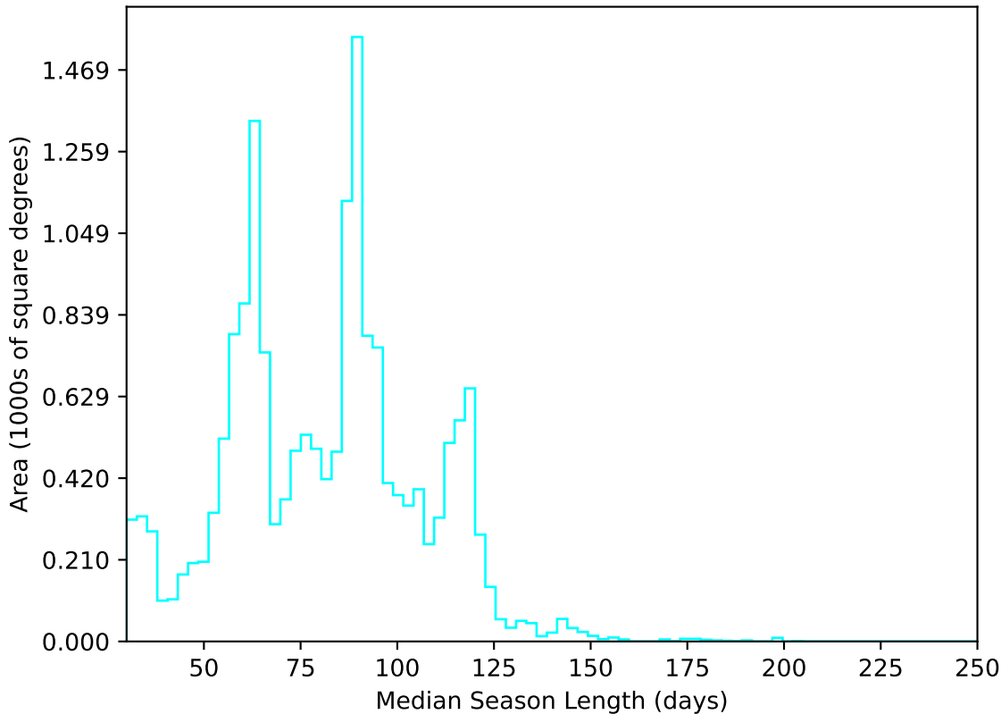
ddf_loaded_half_fl8_v3.4_10yrs WFD u band: Median Season Length
