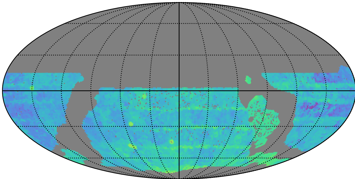
ddf_loaded_half_fl8_v3.4_10yrs WFD r band: Median Season Length
