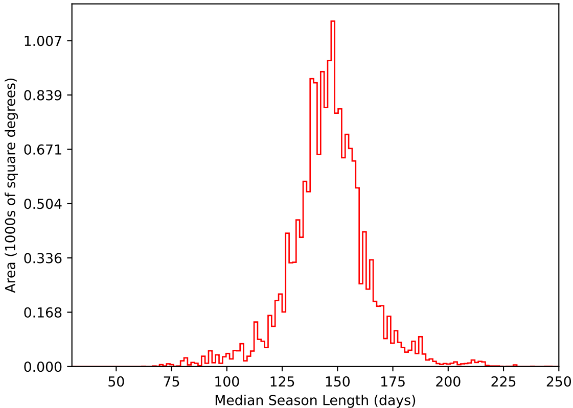
ddf_loaded_half_fl8_v3.4_10yrs WFD i band: Median Season Length
