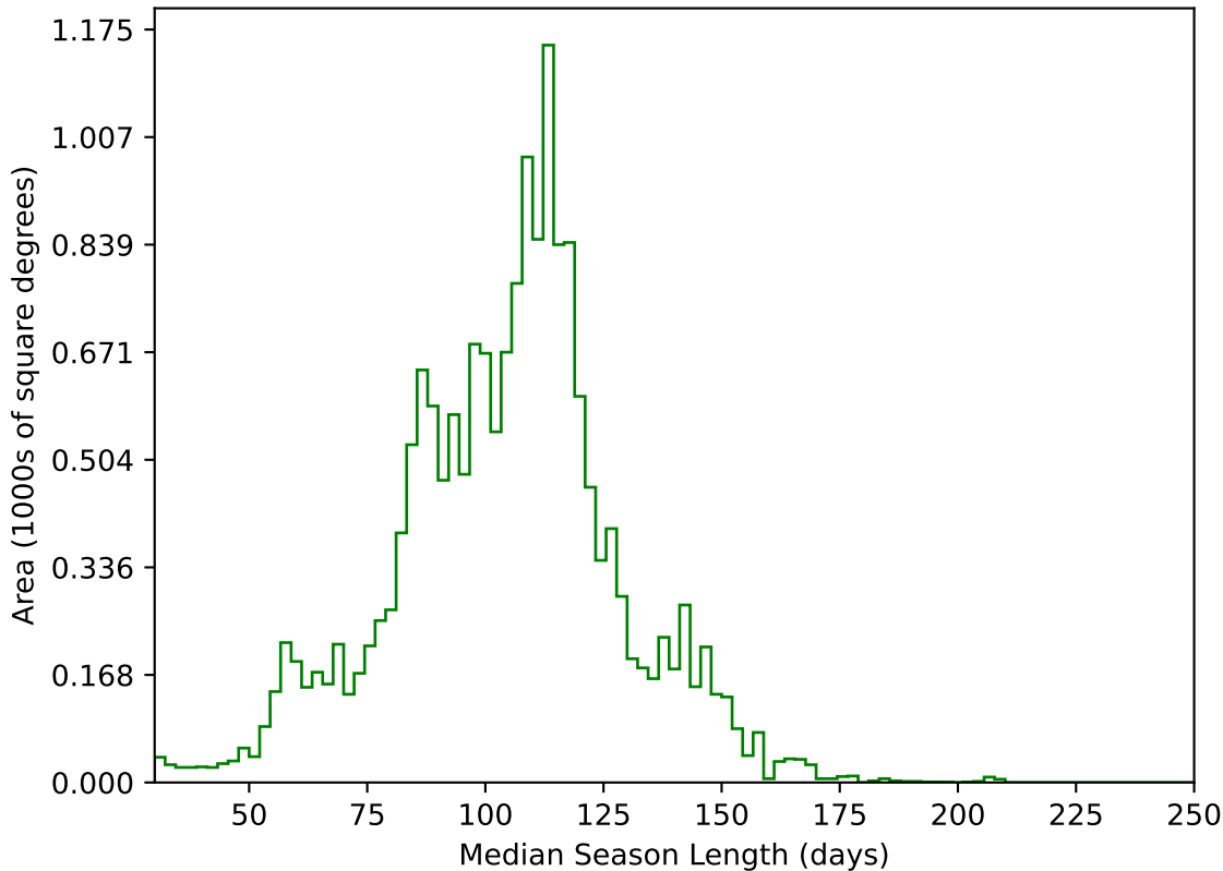
ddf_loaded_half_fl8_v3.4_10yrs WFD g band: Median Season Length
