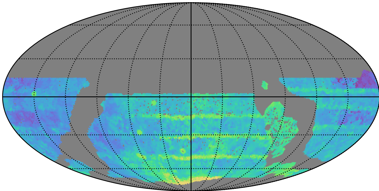
ddf_loaded_half_fl8_v3.4_10yrs WFD all bands: Median Season Length
