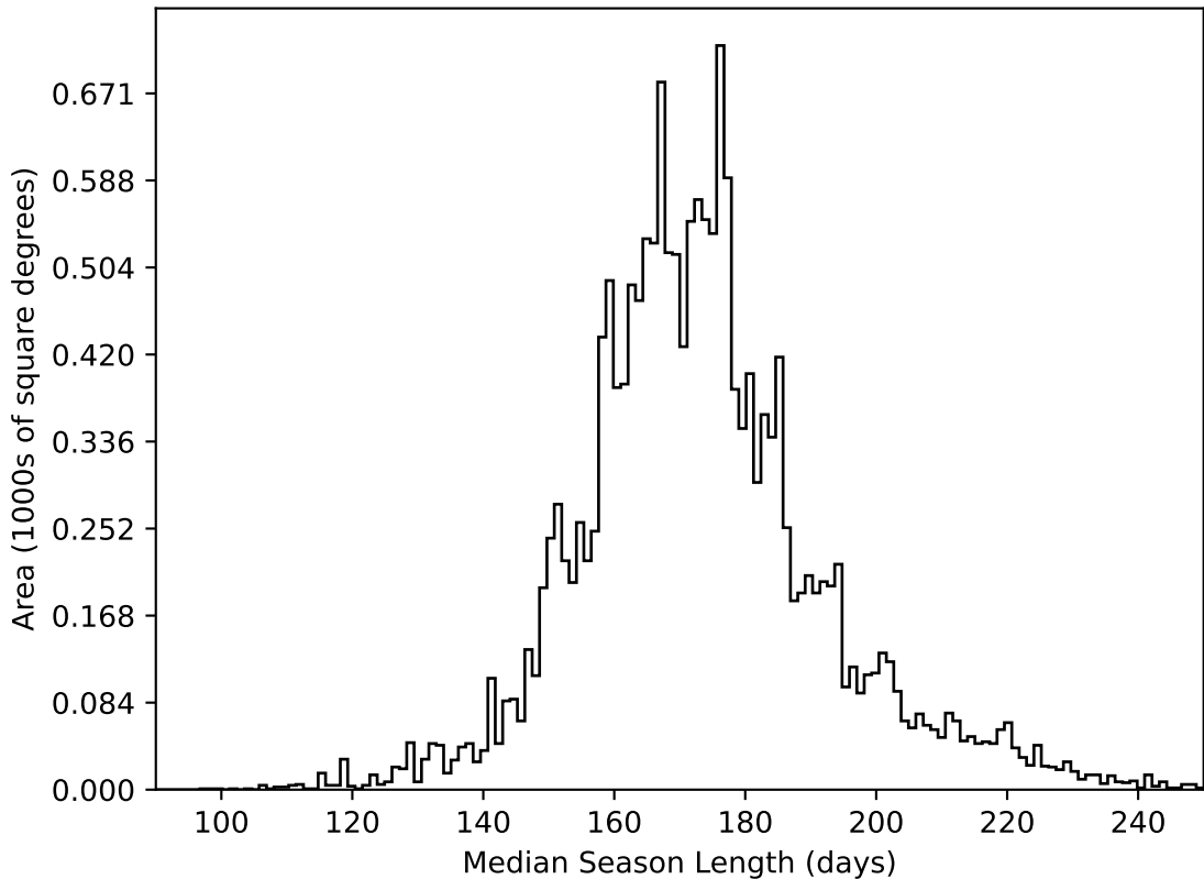
ddf_loaded_half_fl8_v3.4_10yrs WFD all bands: Median Season Length
