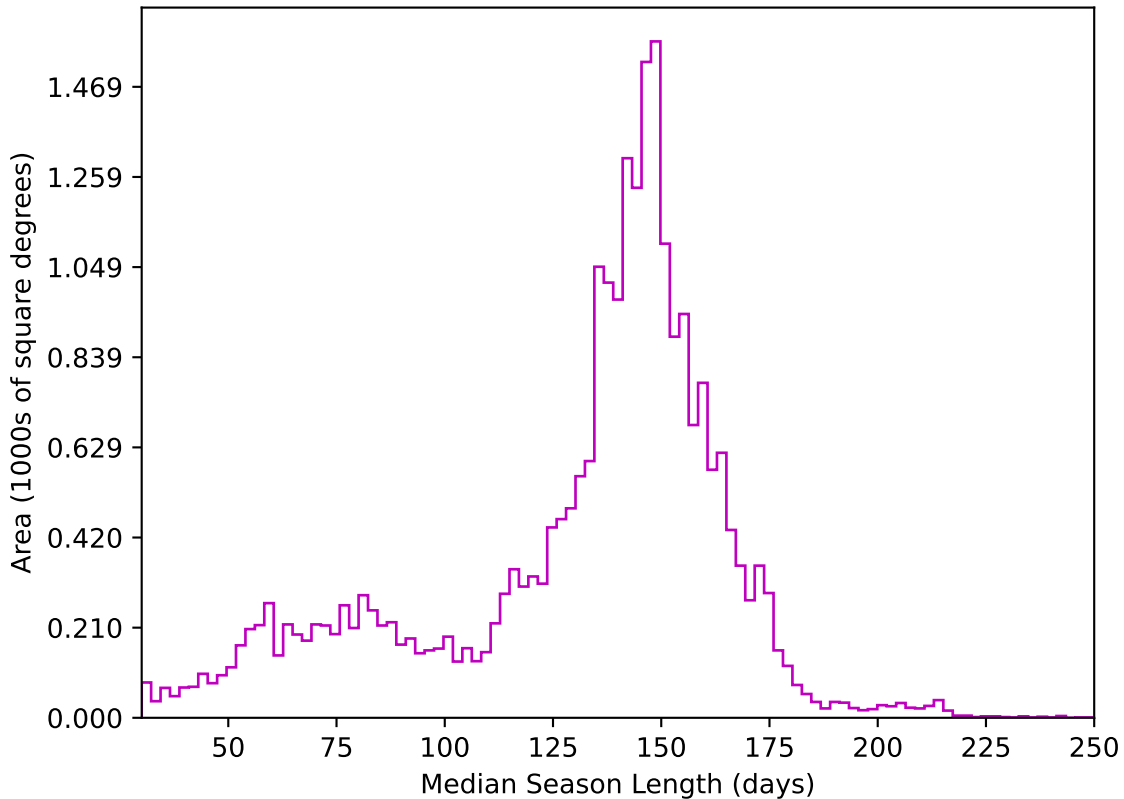
ddf_loaded_half_fl8_v3.4_10yrs All sky z band: Median Season Length
