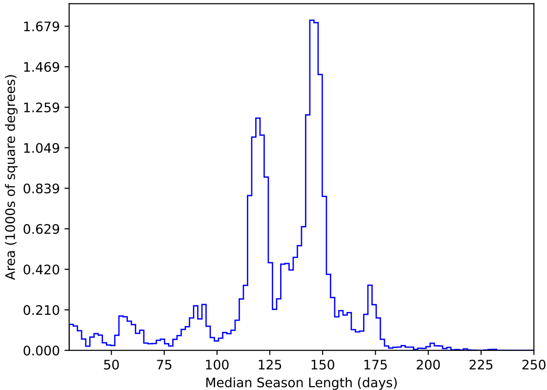
ddf_loaded_half_fl8_v3.4_10yrs All sky y band: Median Season Length
