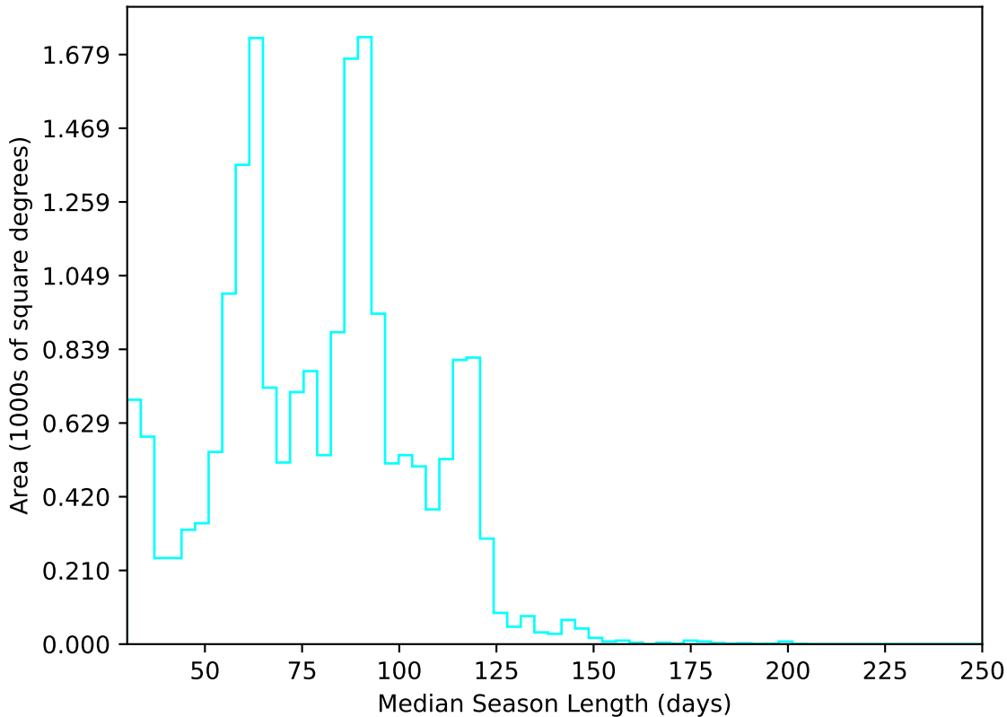
ddf_loaded_half_fl8_v3.4_10yrs All sky u band: Median Season Length
