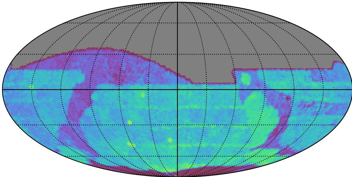
ddf_loaded_half_fl8_v3.4_10yrs All sky r band: Median Season Length
