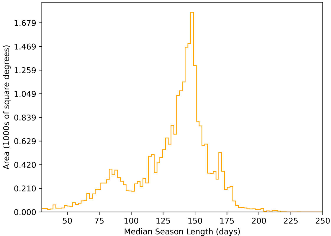
ddf_loaded_half_fl8_v3.4_10yrs All sky r band: Median Season Length
