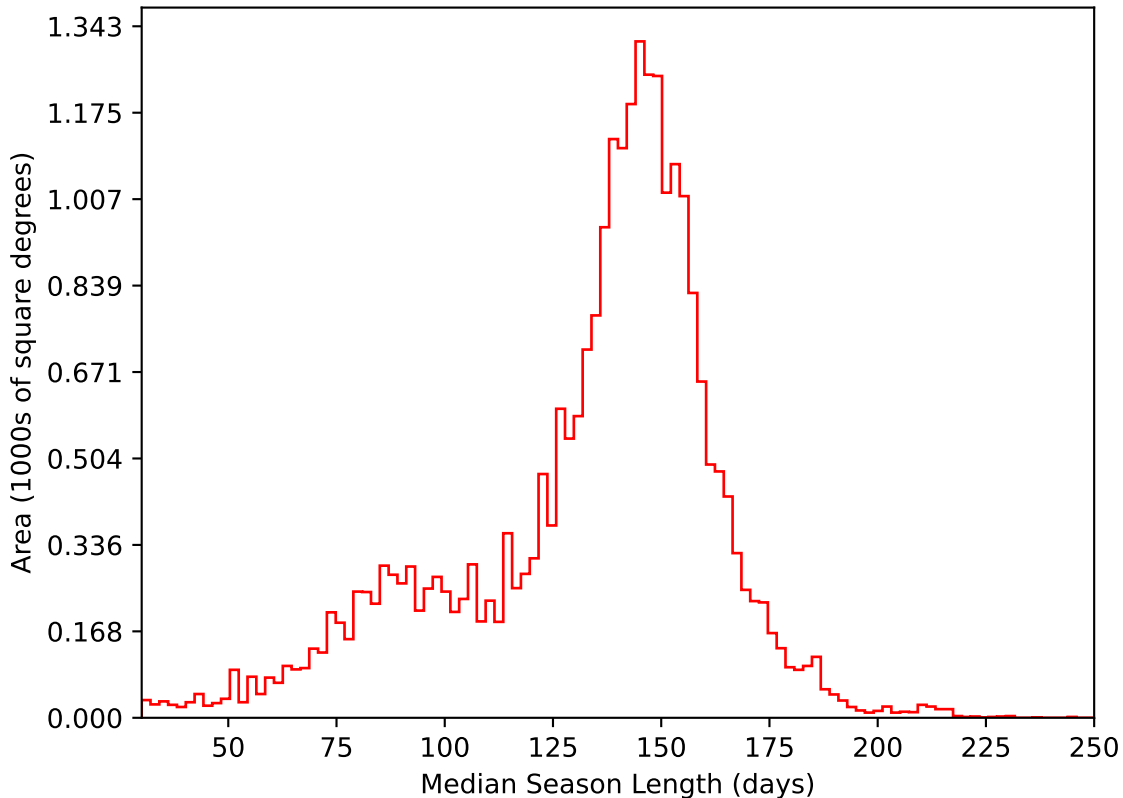
ddf_loaded_half_fl8_v3.4_10yrs All sky i band: Median Season Length
