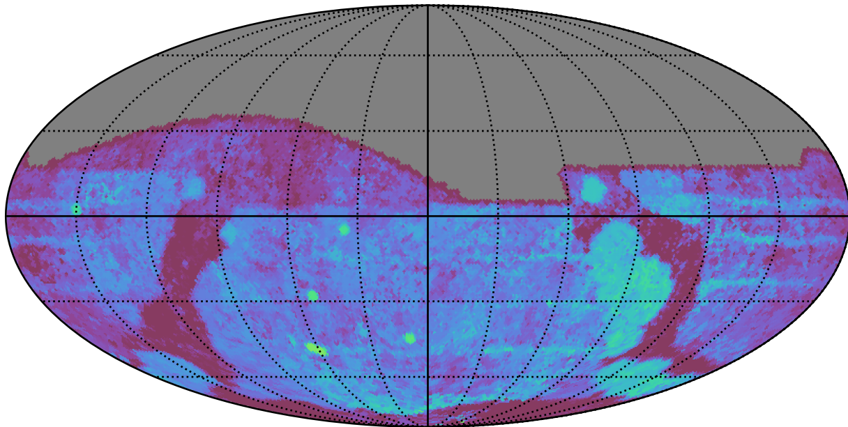
ddf_loaded_half_fl8_v3.4_10yrs All sky g band: Median Season Length
