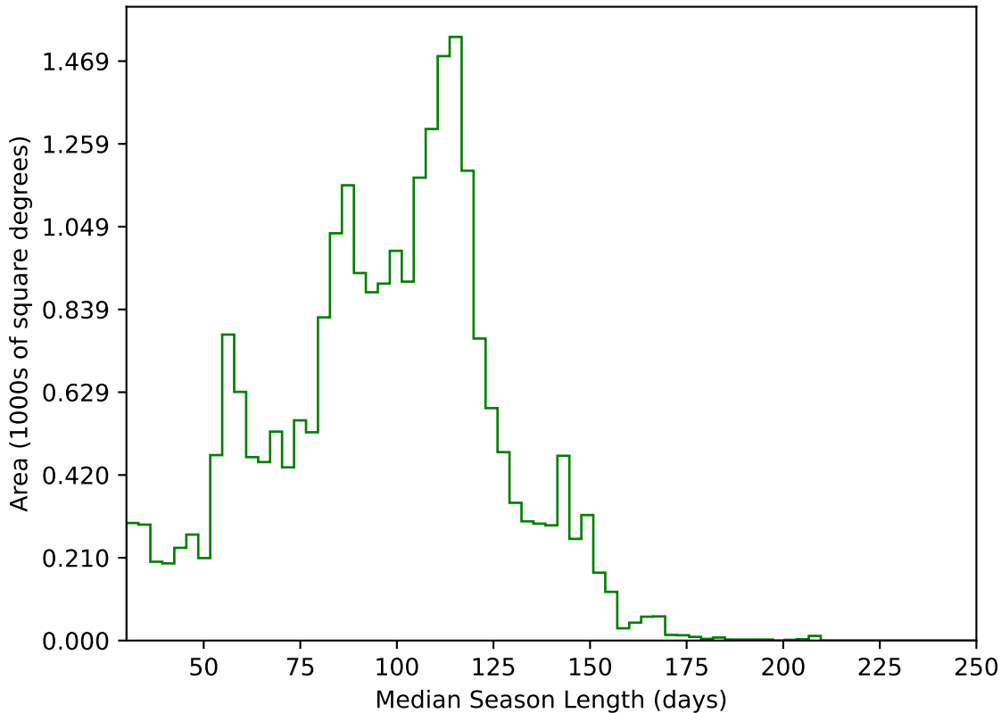
ddf_loaded_half_fl8_v3.4_10yrs All sky g band: Median Season Length
