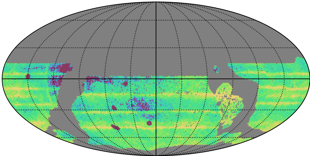
ddf_loaded_half_fl8_v3.4_10yrs WFD: Median Intra-Night Gap
