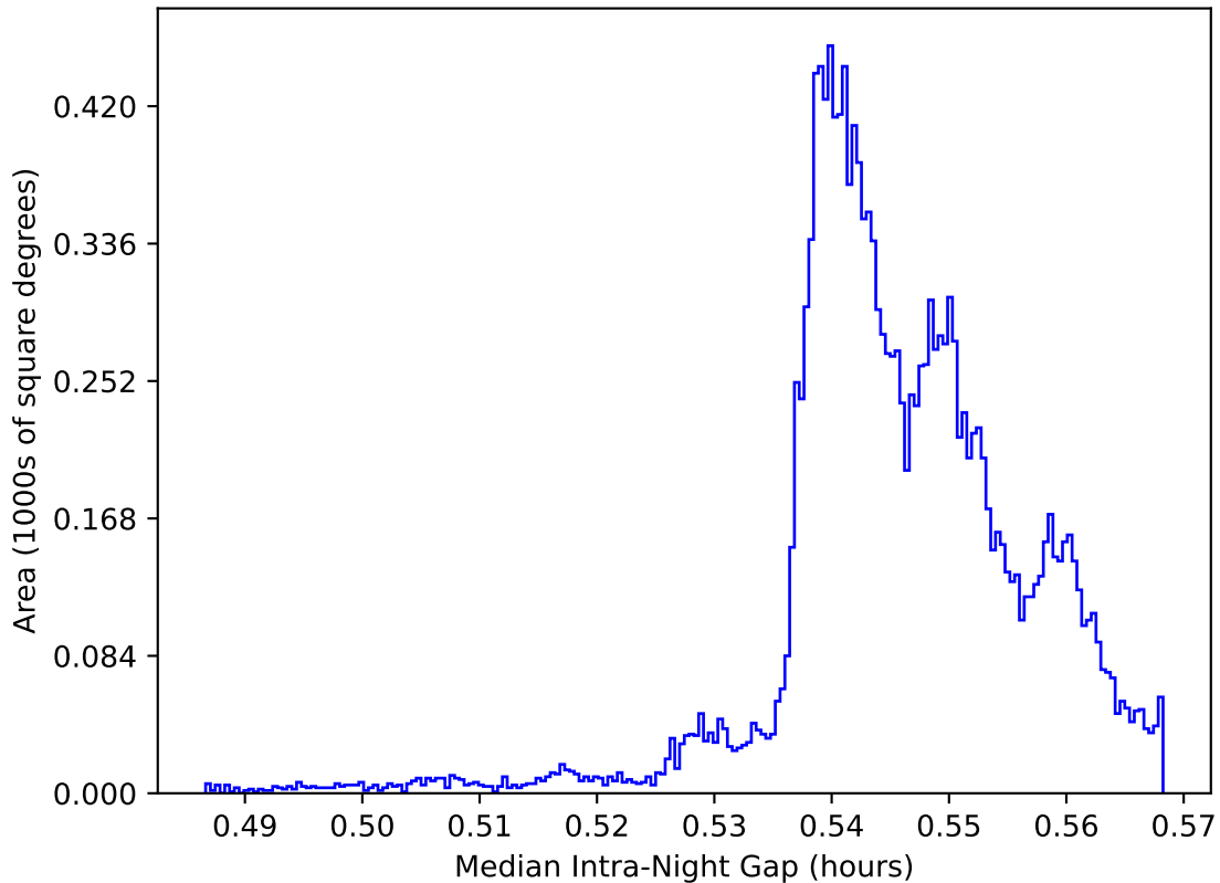
ddf_loaded_half_fl8_v3.4_10yrs WFD: Median Intra-Night Gap
