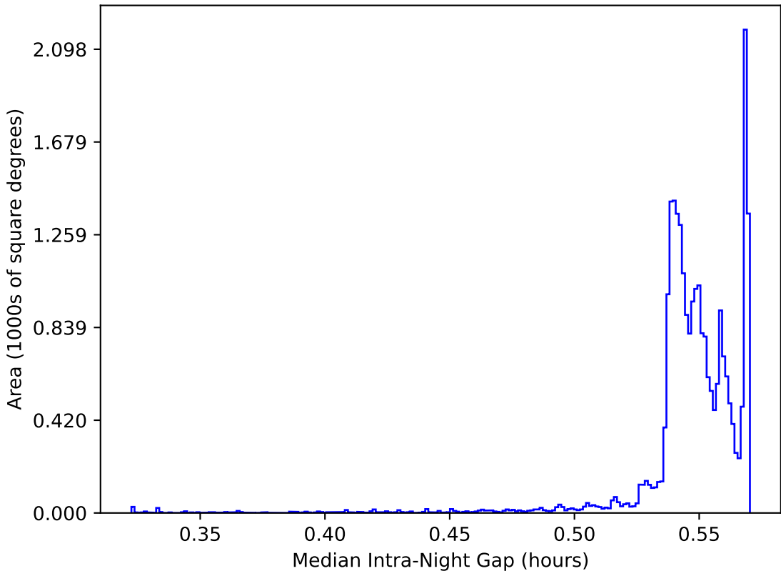
ddf_loaded_half_fl8_v3.4_10yrs All sky: Median Intra-Night Gap
