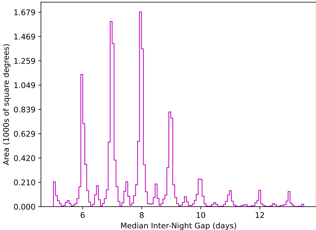
ddf_loaded_half_fl8_v3.4_10yrs WFD z band: Median Inter-Night Gap
