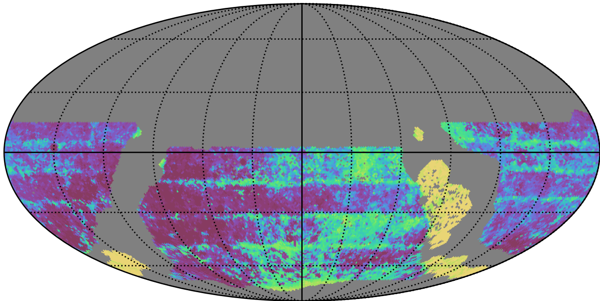
ddf_loaded_half_fl8_v3.4_10yrs WFD y band: Median Inter-Night Gap
