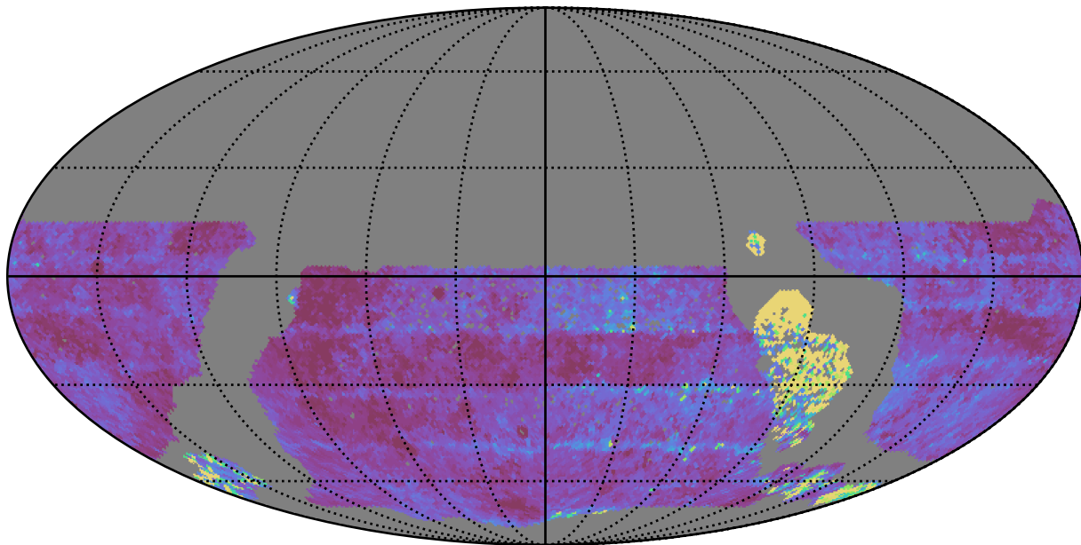
ddf_loaded_half_fl8_v3.4_10yrs WFD u band: Median Inter-Night Gap
