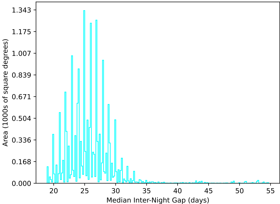
ddf_loaded_half_fl8_v3.4_10yrs WFD u band: Median Inter-Night Gap
