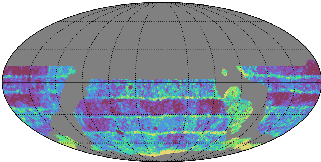
ddf_loaded_half_fl8_v3.4_10yrs WFD r band: Median Inter-Night Gap
