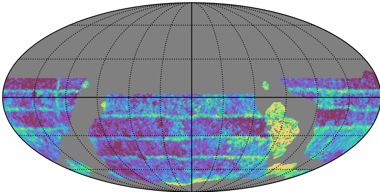
ddf_loaded_half_fl8_v3.4_10yrs WFD i band: Median Inter-Night Gap
