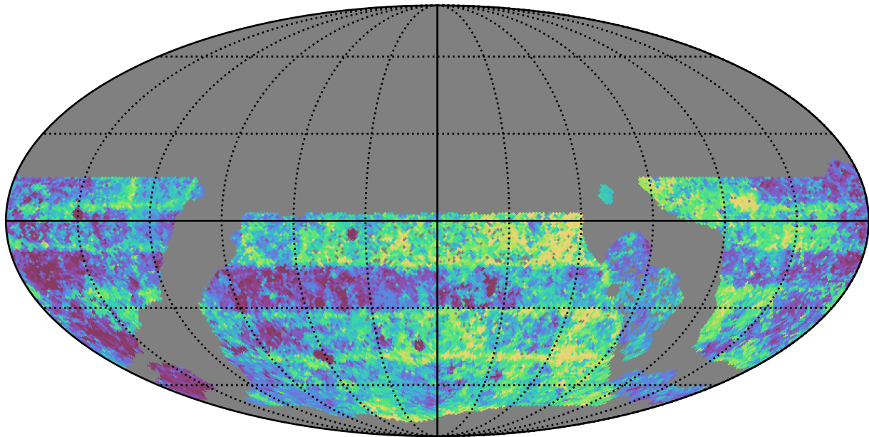
ddf_loaded_half_fl8_v3.4_10yrs WFD g band: Median Inter-Night Gap
