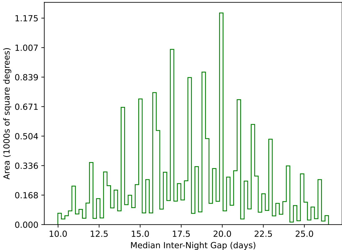
ddf_loaded_half_fl8_v3.4_10yrs WFD g band: Median Inter-Night Gap
