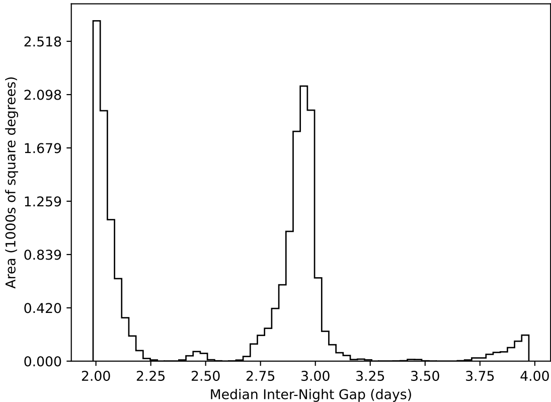
ddf_loaded_half_fl8_v3.4_10yrs WFD all bands: Median Inter-Night Gap
