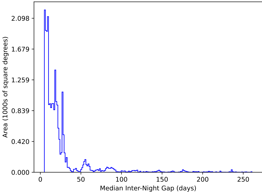
ddf_loaded_half_fl8_v3.4_10yrs All sky y band: Median Inter-Night Gap
