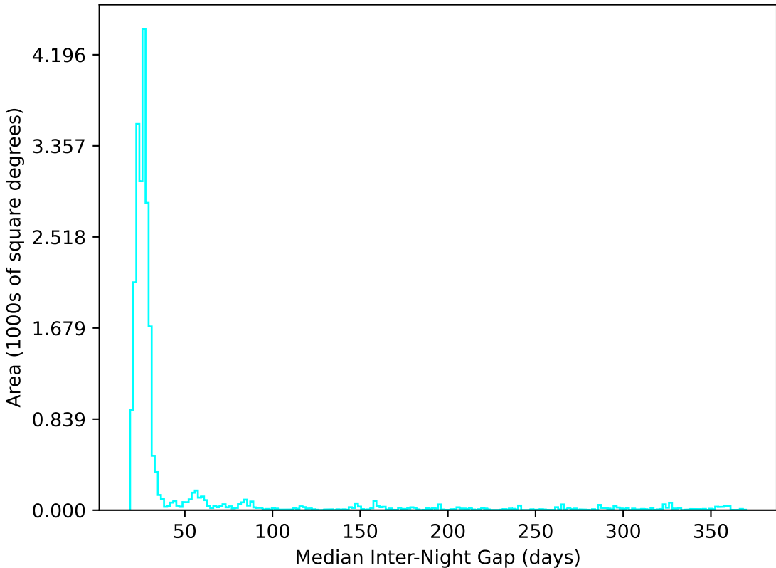
ddf_loaded_half_fl8_v3.4_10yrs All sky u band: Median Inter-Night Gap
