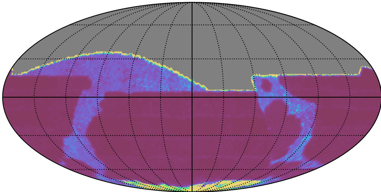
ddf_loaded_half_fl8_v3.4_10yrs All sky r band: Median Inter-Night Gap
