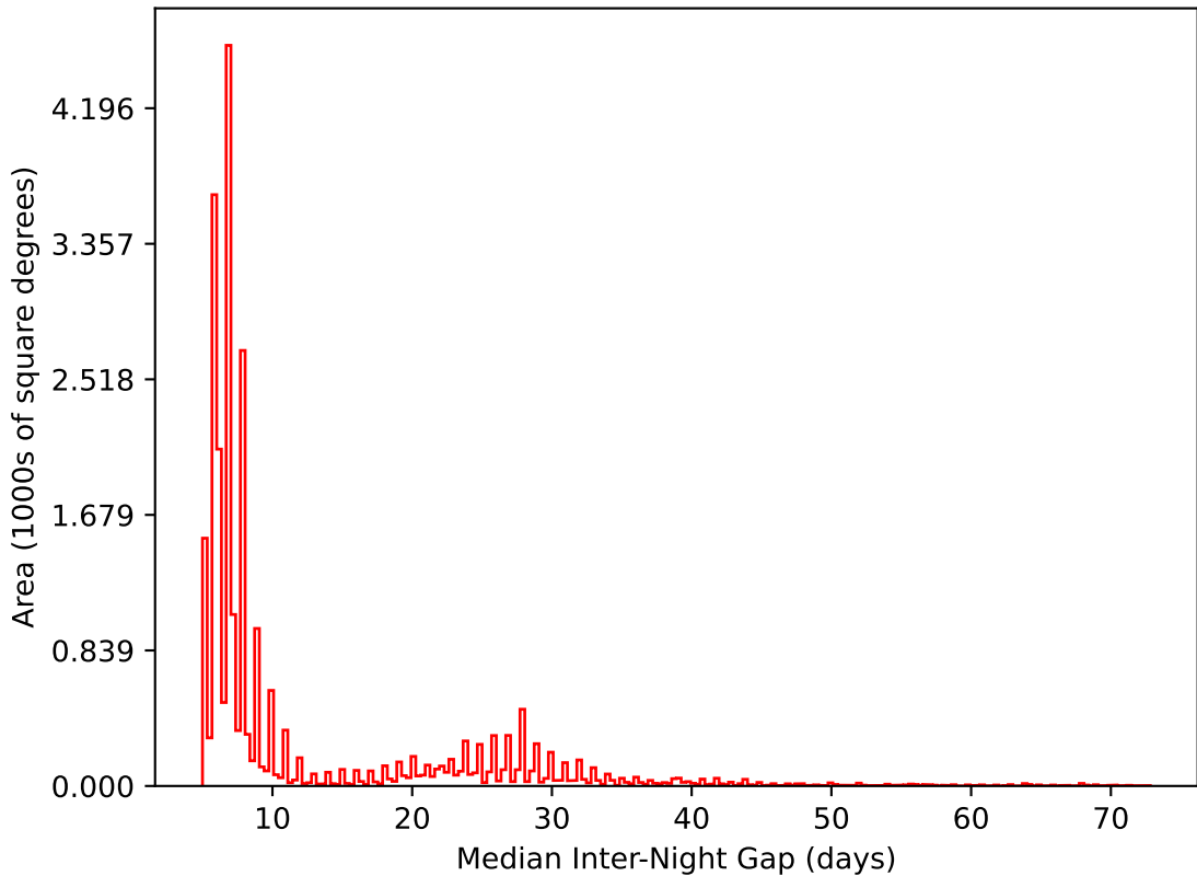
ddf_loaded_half_fl8_v3.4_10yrs All sky i band: Median Inter-Night Gap
