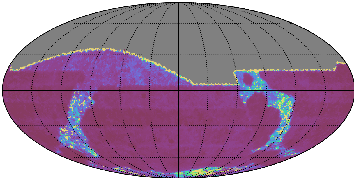
ddf_loaded_half_fl8_v3.4_10yrs All sky g band: Median Inter-Night Gap
