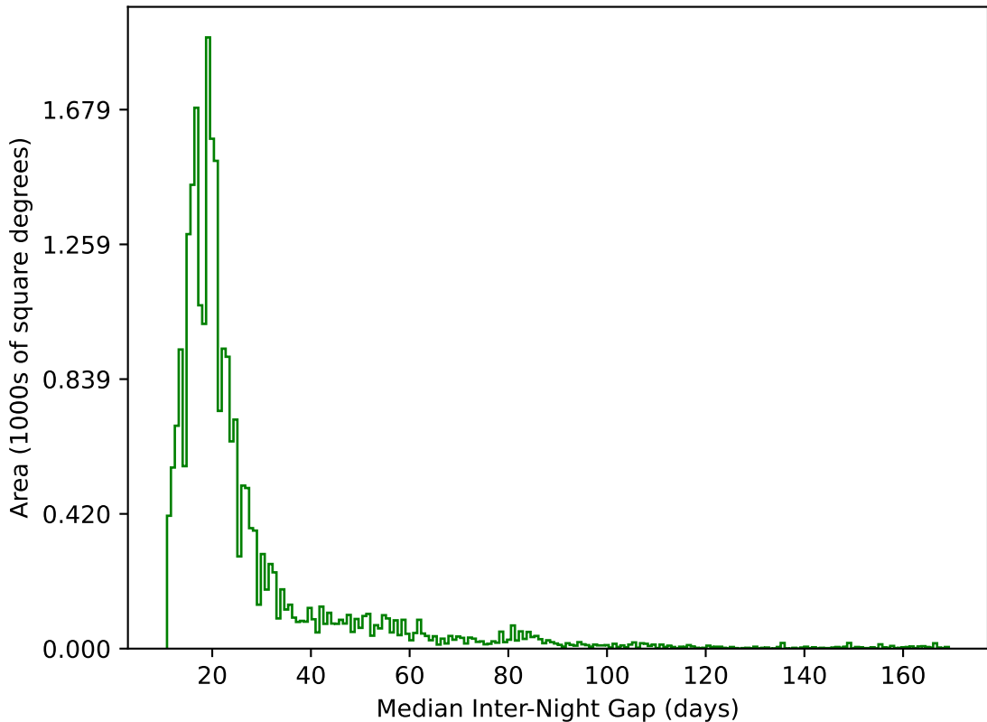
ddf_loaded_half_fl8_v3.4_10yrs All sky g band: Median Inter-Night Gap
