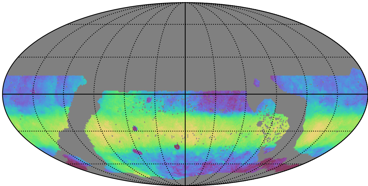
ddf_loaded_half_fl8_v3.4_10yrs WFD z band: Median HA
