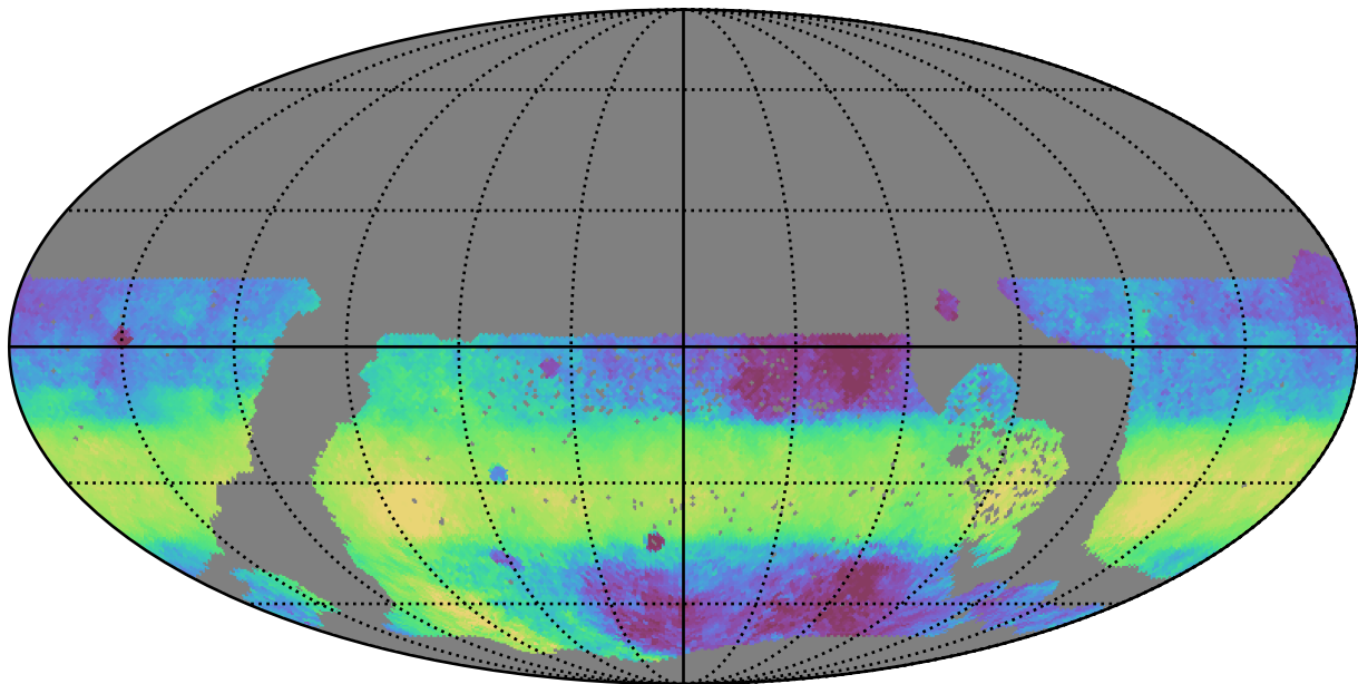
ddf_loaded_half_fl8_v3.4_10yrs WFD y band: Median HA
