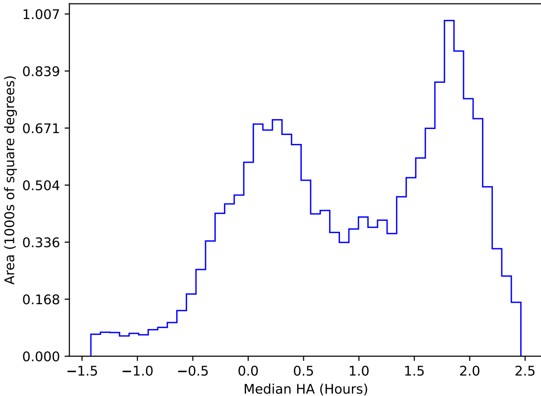
ddf_loaded_half_fl8_v3.4_10yrs WFD u band: Median HA
