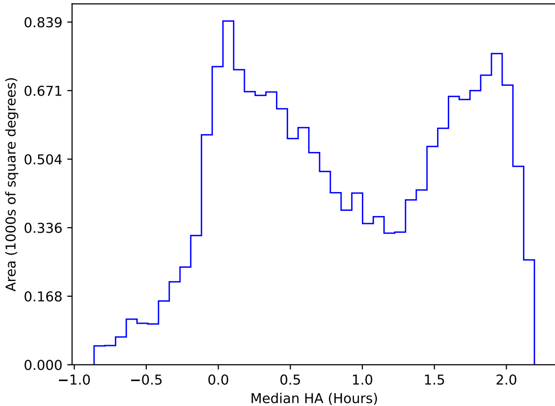
ddf_loaded_half_fl8_v3.4_10yrs WFD r band: Median HA
