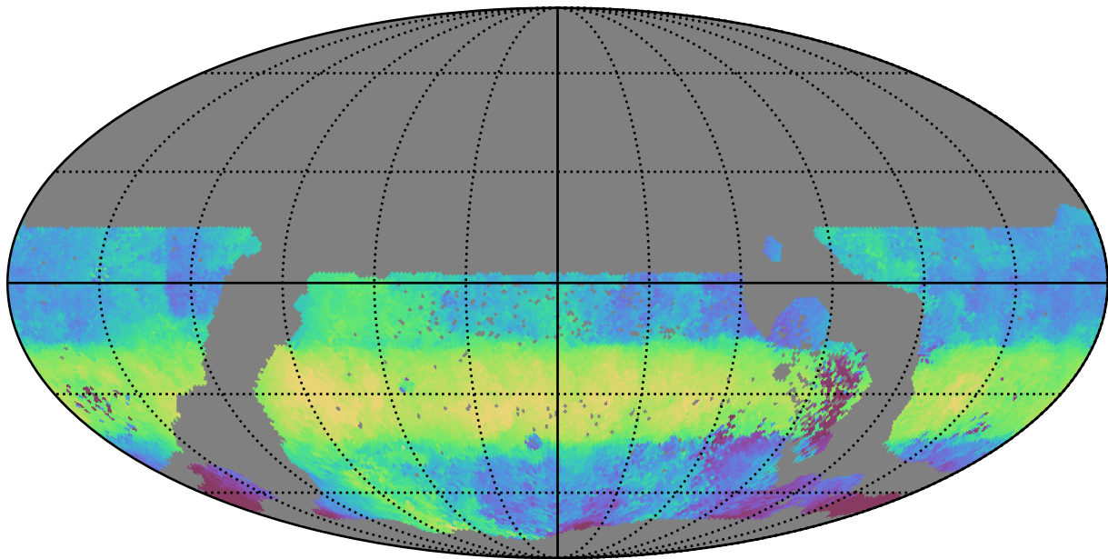
ddf_loaded_half_fl8_v3.4_10yrs WFD g band: Median HA
