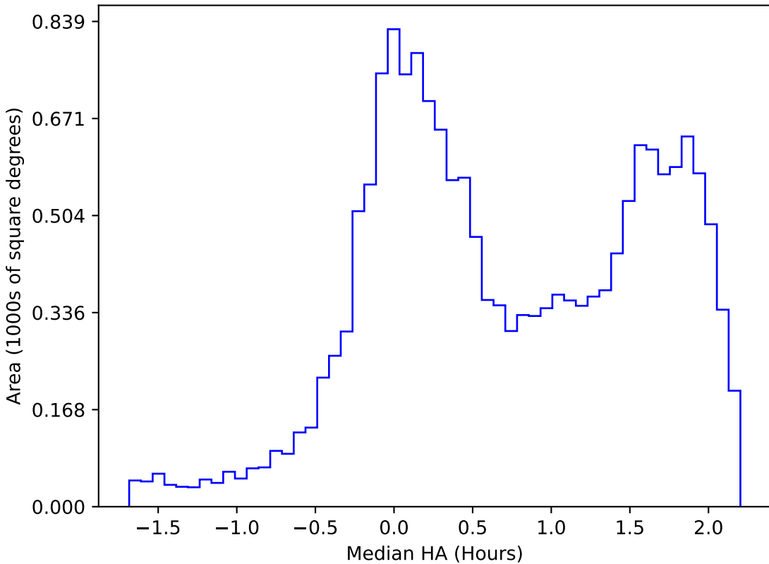
ddf_loaded_half_fl8_v3.4_10yrs WFD g band: Median HA
