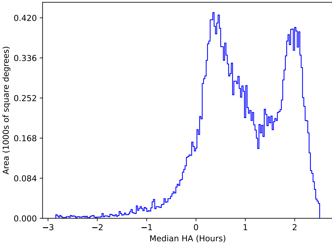
ddf_loaded_half_fl8_v3.4_10yrs All sky z band: Median HA
