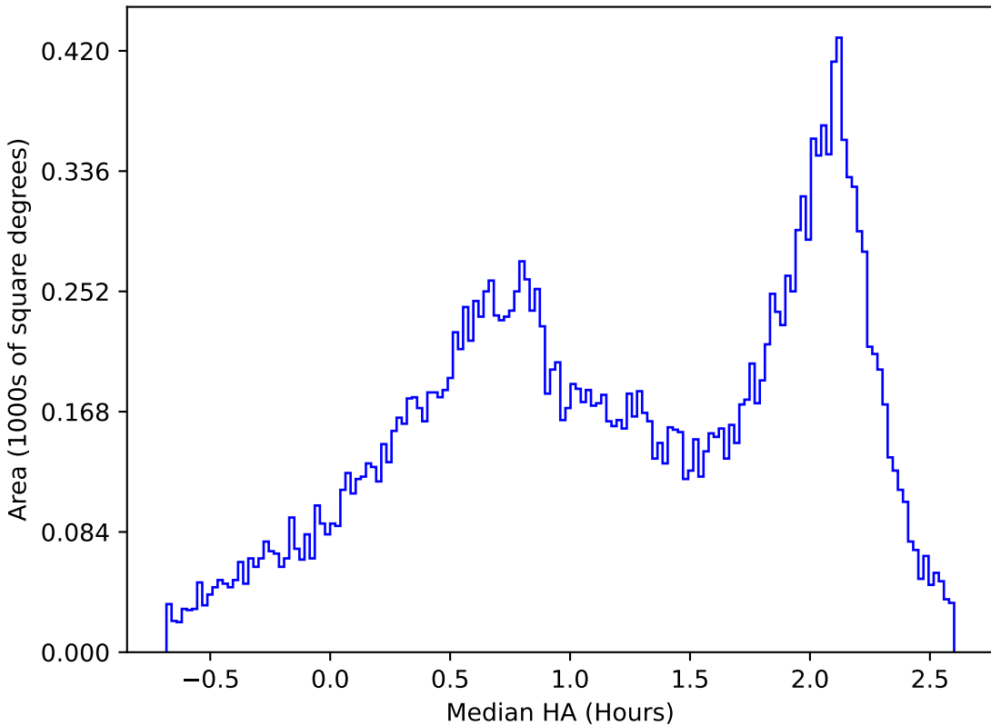
ddf_loaded_half_fl8_v3.4_10yrs All sky y band: Median HA
